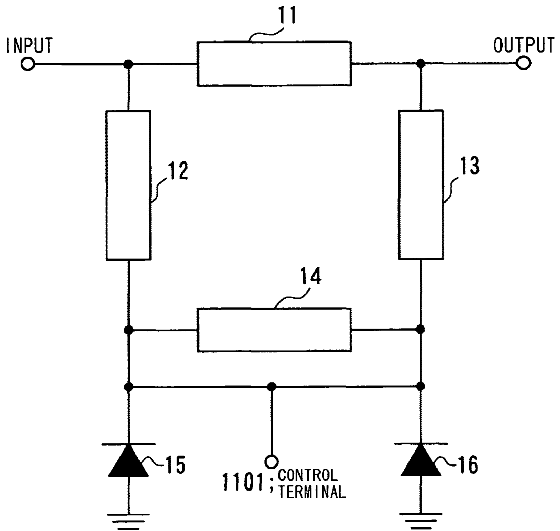
PHASE SHIFTER
